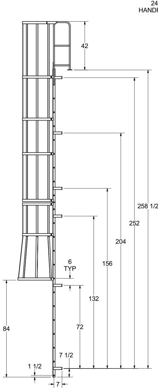
DETAIL A
